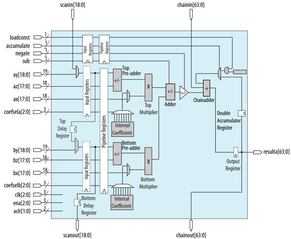
Figure 3. The 18 × 18 Sum of 2 Mode Architecture
