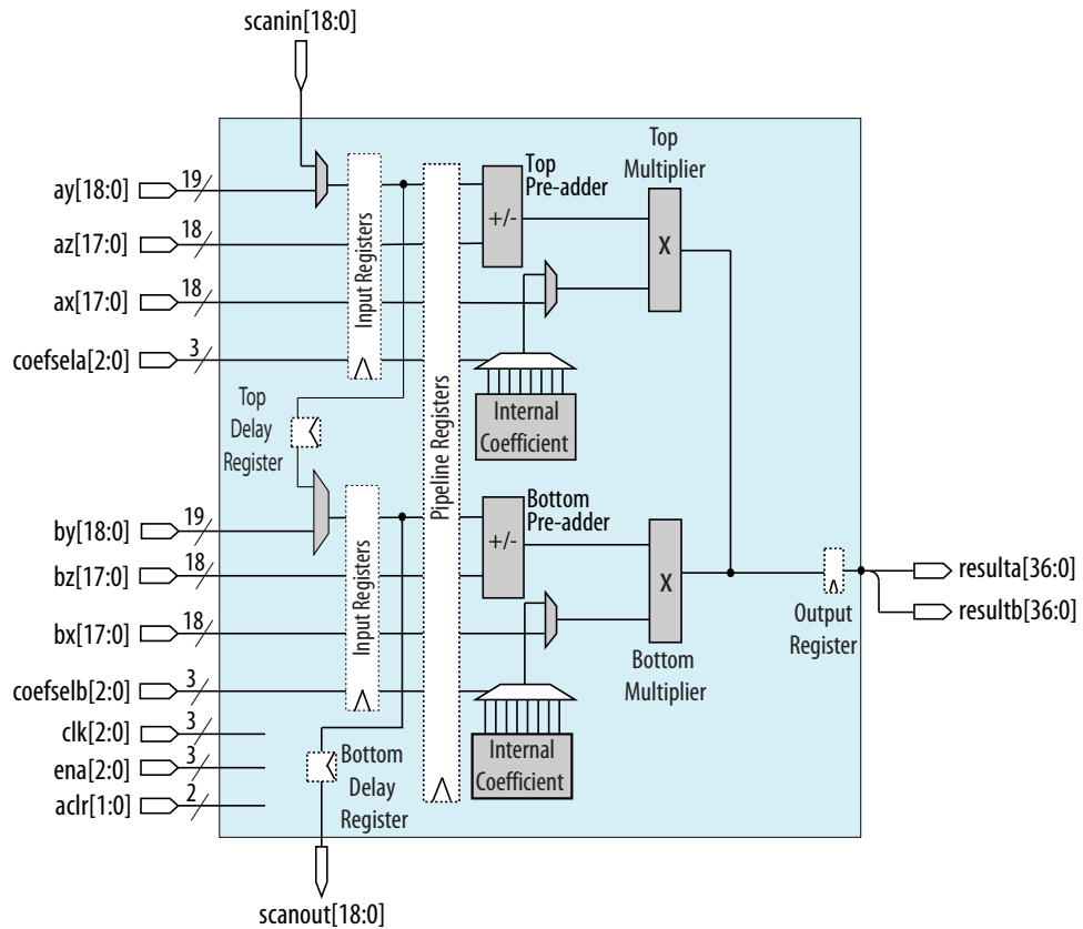
Figure 2. The 18 × 18 Full Mode Architecture
