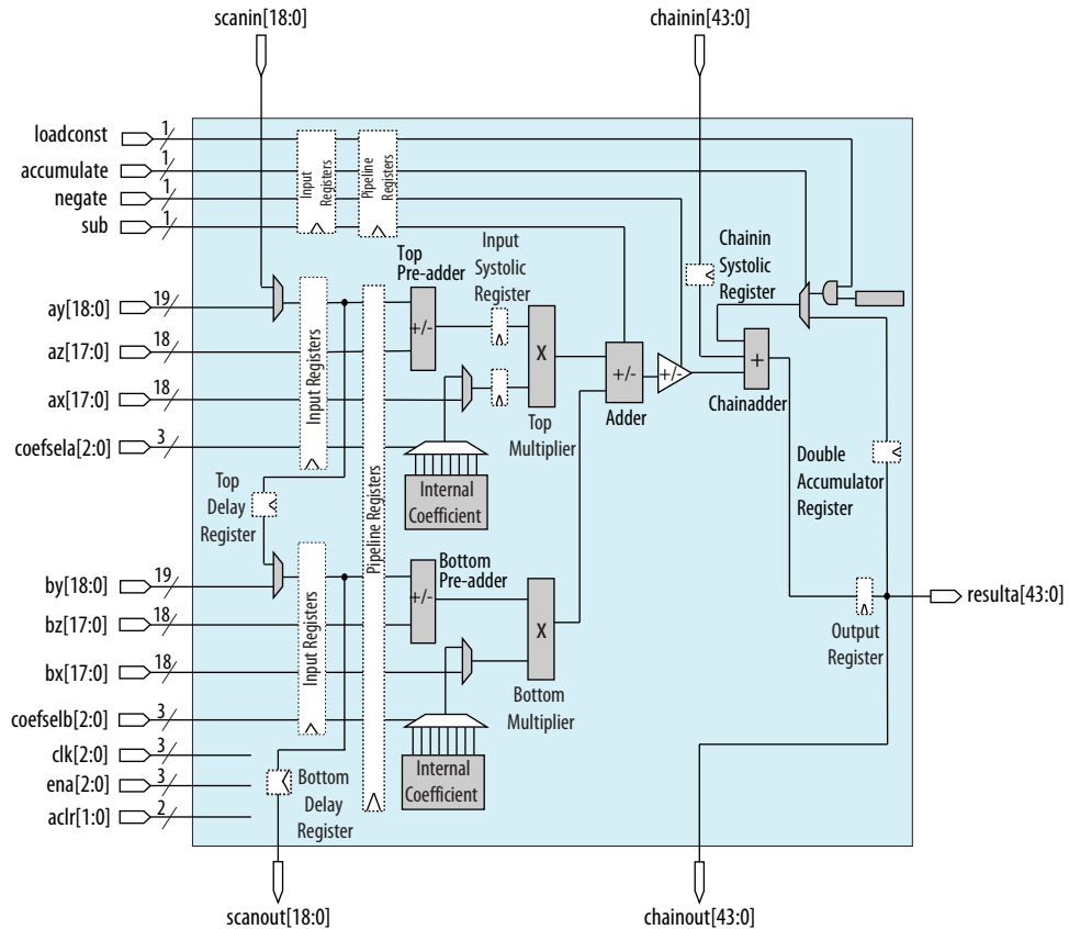
Figure 5. The 18 × 18 Systolic Mode Architecture
