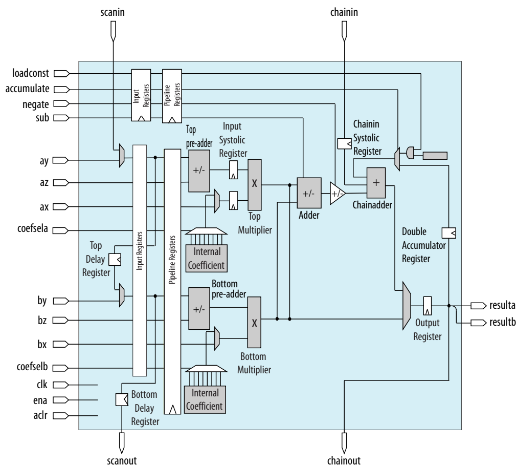
Figure 1. Cyclone 10 GX Native Fixed Point DSP IP Core Functional Block Diagram
