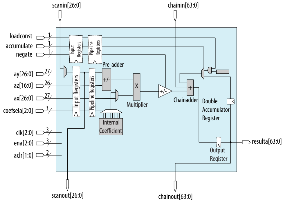
Figure 6. The 27 × 27 Mode Architecture
