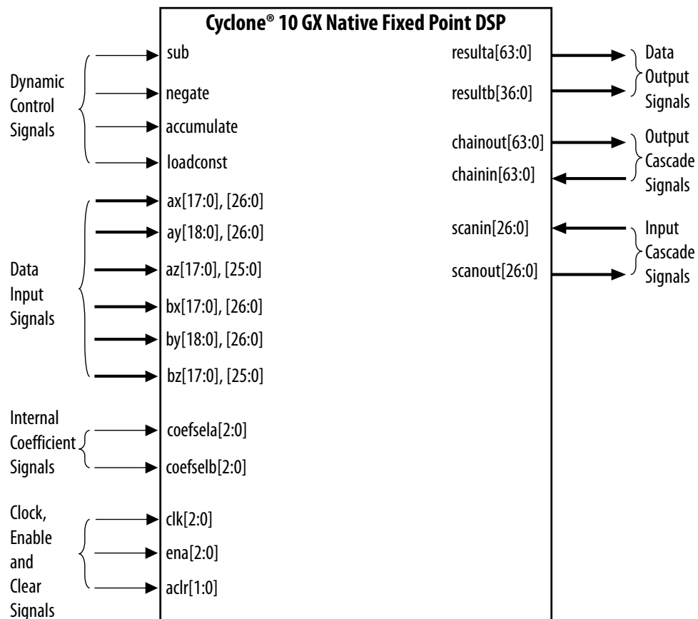
Figure 7. Cyclone 10 GX Native Fixed Point DSP IP Core Signals
