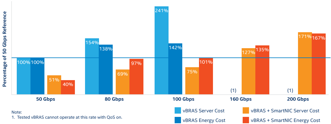
Figure 10. Total Cost of Server as a Percentage of Reference (50 Gbps) Total Cost of Energy as a Percentage of Reference (50 Gbps) after 3 Years
