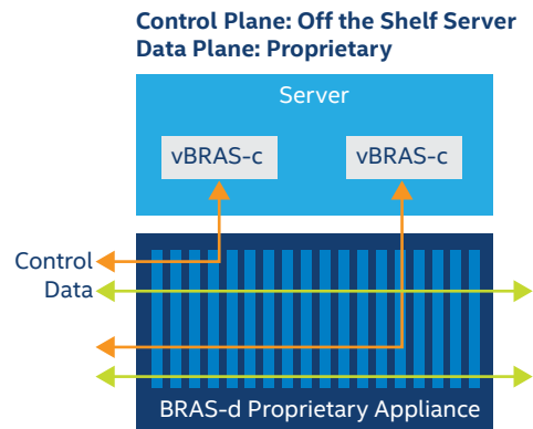
Figure 12. Alternate CUPS Implementation
