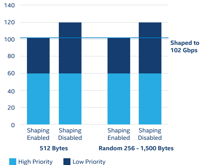
Figure 7. Data Plane Node Performance
