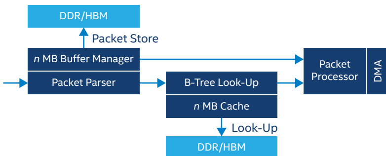
Figure 4. Packet-Forwarding FPGA Design
