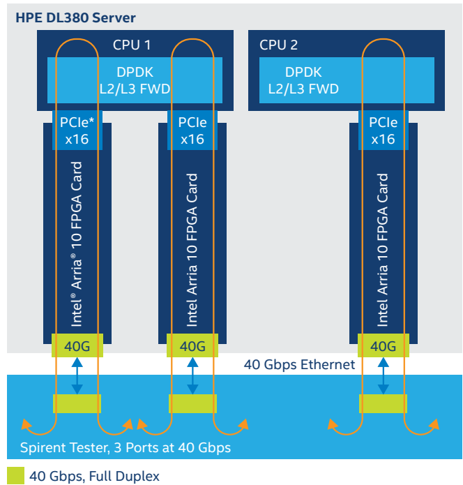
Figure 6. DL380 Server Setup with 3 FPGA SmartNICs Supporting 120 Gbps with QoS and Traffic Shaping
