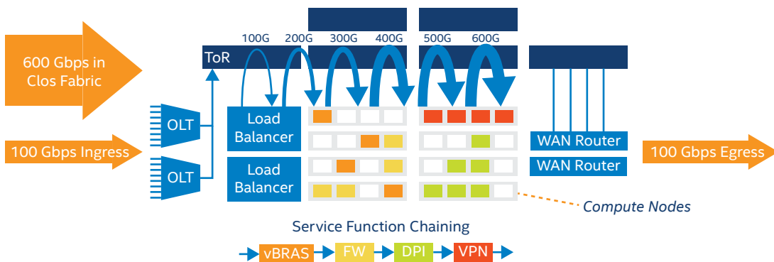
Figure 1. Inefficient vBRAS Deployment Example
