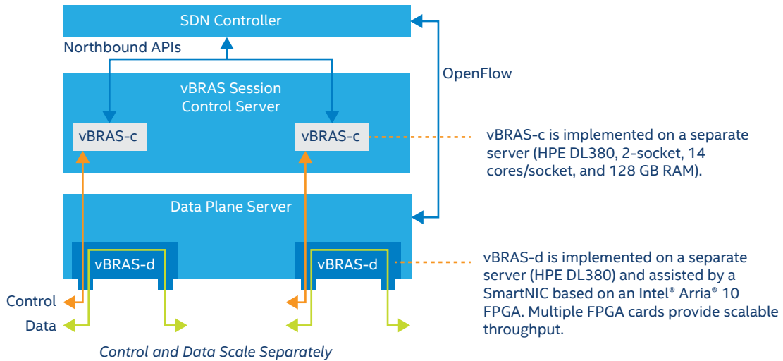
Figure 3. SDN-Inspired Split vBRAS
